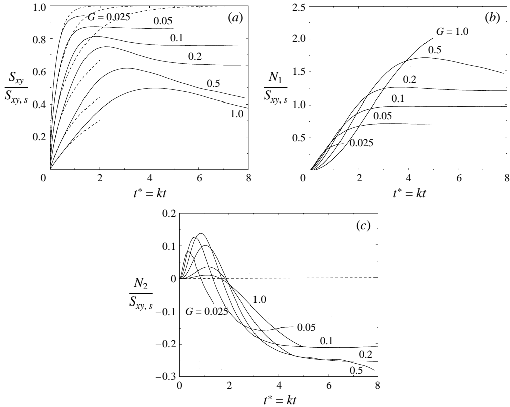
FIGURE 12. Transient profiles of normalized particle (a) shear stress, (b) first normal-stress difference, and (c) second normal-stress difference for initially spherical capsules with \lambda = 1 . Dashed lines indicate predictions of linear perturbation theory.
