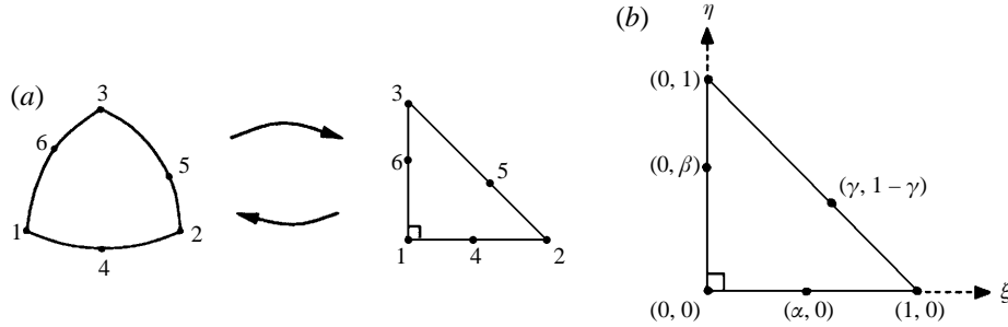
FIGURE 3. (a) Mapping of a curved surface triangle onto the parametric right triangle. (b) The six nodes of the local parametric triangle.
