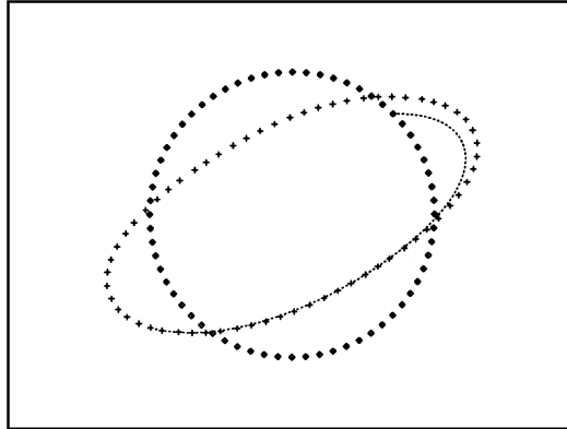
FIGURE 10. Trajectory of a single material point superimposed on initial and final contours of an initially spherical capsule with \lambda = 1.0 deformed at G = 0.2 . Trajectory reflects initial deformation of capsule and subsequent tank-treading at a steady configuration.
